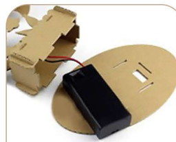
Bottom mounted battery 从底部安装电池
