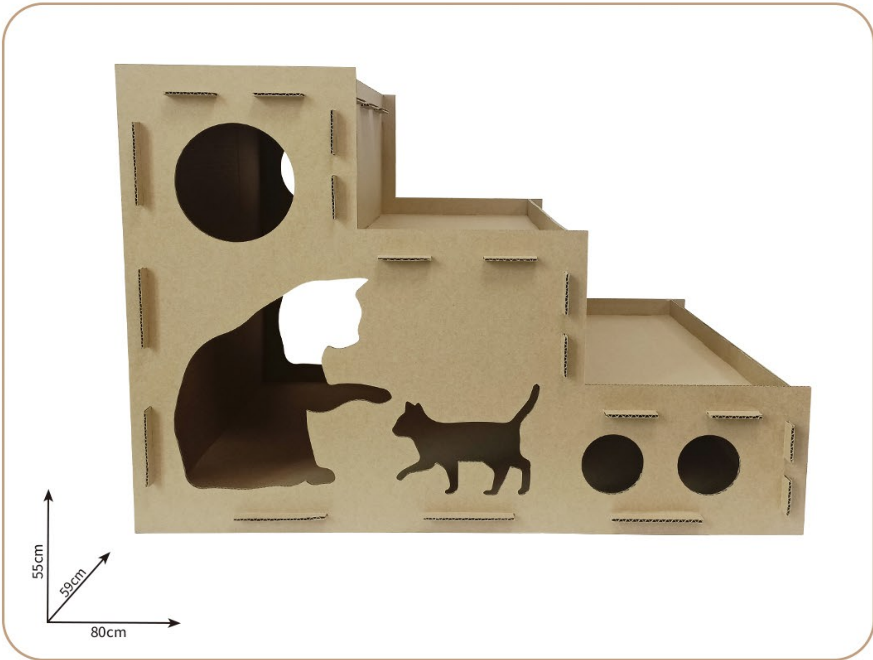
CAT PET HOUSE ITEM NO. : CS160 MODEL SIZE: 80 × 59 × 55cm MATERIAL: CORRUGATED MOQ : 3000PCS SHEET SIZE & QTY : 110cm × 60 cm / 4 (sheets)
